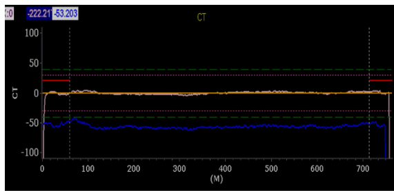
Fig.8. Coiling temperature after process optimization.
