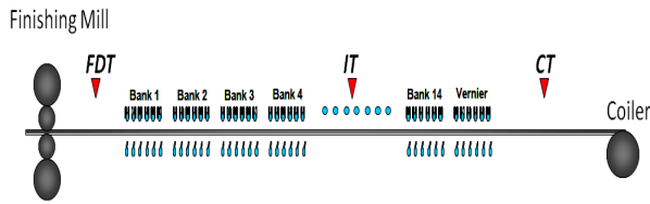
Fig.1. Layout of the ROT.
