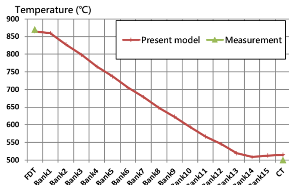
Fig.6. Predicted temperature at strip tail end.
