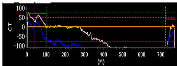
Fig.3. Coiling temperature before process optimization.
