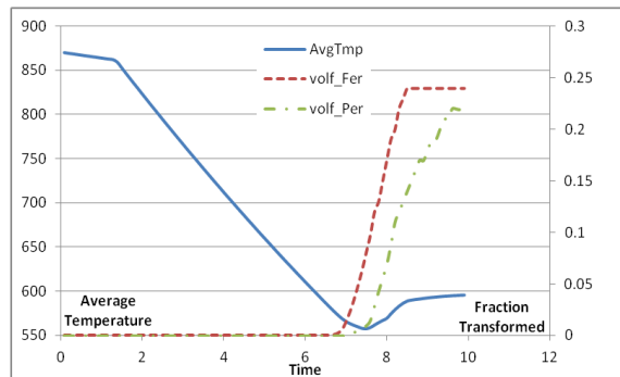
Fig.5. Predicted temperature and phase evolution of medium carbon steel.
