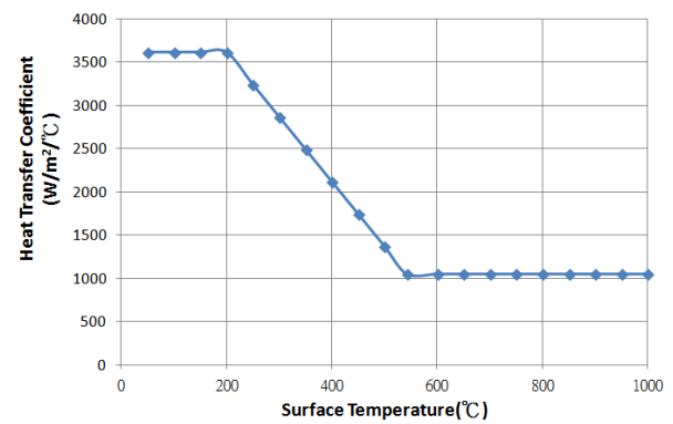
Fig.2. Heat transfer coefficient for the water cooling.
