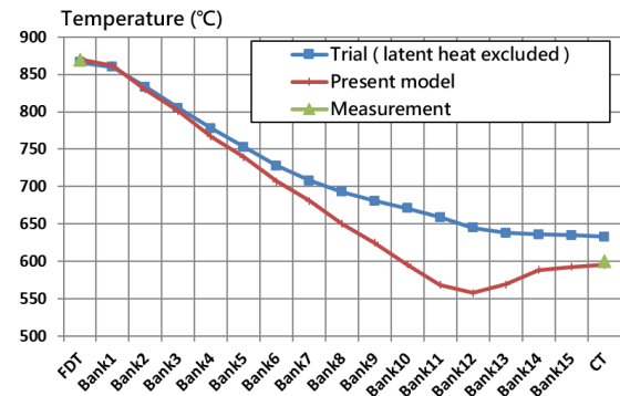
Fig.4. Predicted temperature at strip head end.
