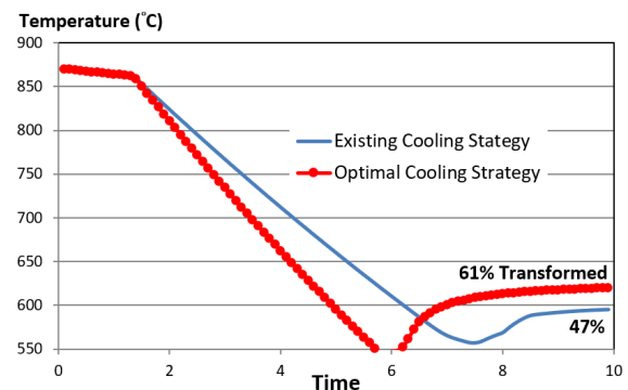
Fig.7. Optimal cooling strategy for medium carbon steel.
