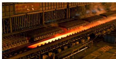
層流冷卻
