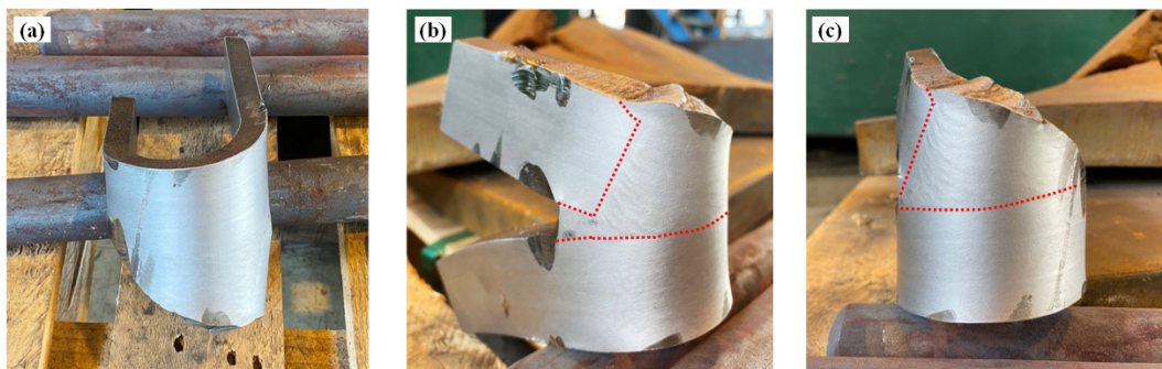
Fig.11. Results of the bending tests for node welding zone. The area indicated by the red dotted line is the weld bead.
