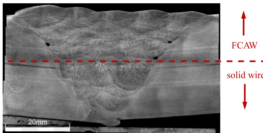
Fig.14. The macro-metallography of simulated GMAW weldment (Upper is flux cored wire ; Bottom is GMAW-solid-wire)
