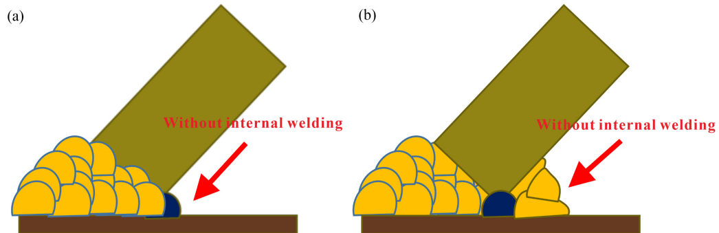
Fig.1. Two different welding designs of nodes: (a) in Europe and (b) in Taiwan. The blue area is the first bead.
