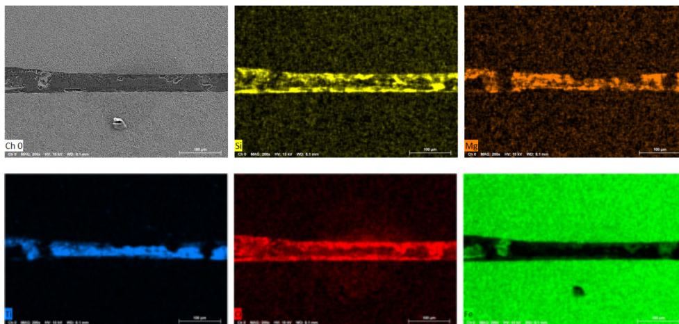
Fig.12. EDS mapping result for simulated weld surface after strong surface grinding. (using NSSW FCAW wire)
