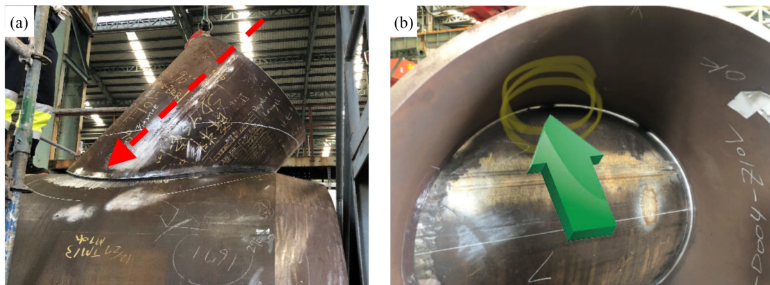
Fig.2. (a) The location of the inner weld direction on the node from an external perspective. (b) The location of the inner weld direction on the node from an internal perspective. The welder must overcome the narrow space and angle limitations.
