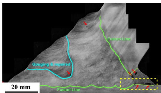
Fig.6. Macro cross-section metallography of welding zone. Defects are indicated by red arrows.
