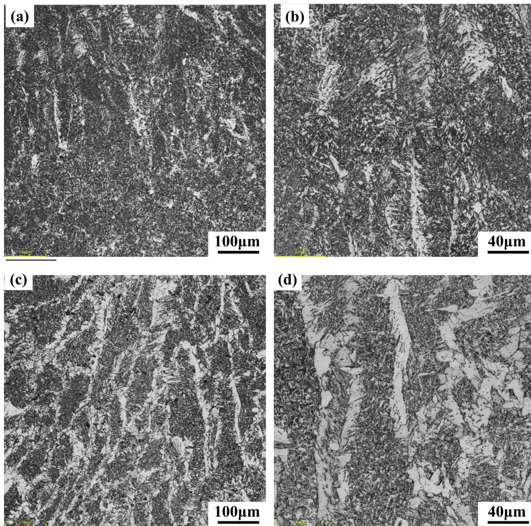
Fig.15. The metallography of weldment (a) FCAW; (b) FCAW; (c) MCAW; (d) MCAW.
