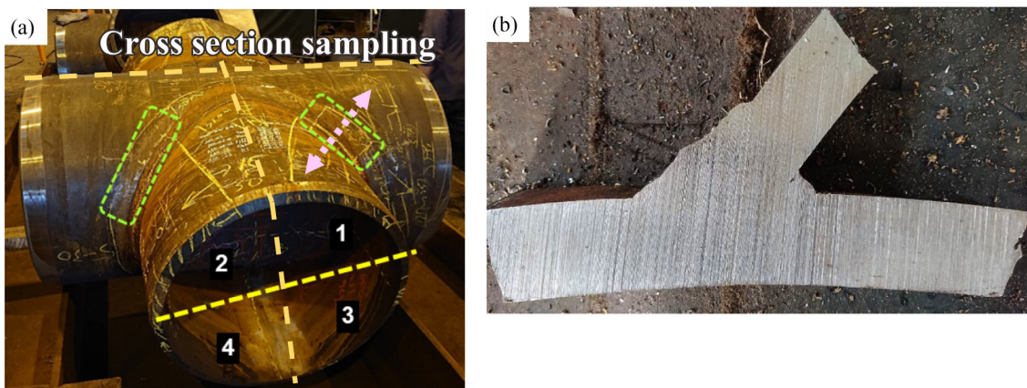
Fig.4. Sampling preparation of the welded node. (a) cutting indications, (b) cross-section of the weld.
