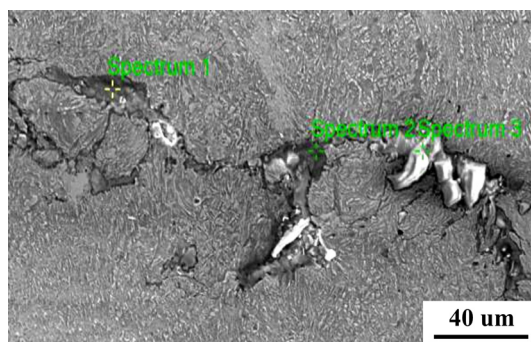
Fig.7. Micro-metallographic of the poor fusion zone indicated in the yellow box area in figure 6.
