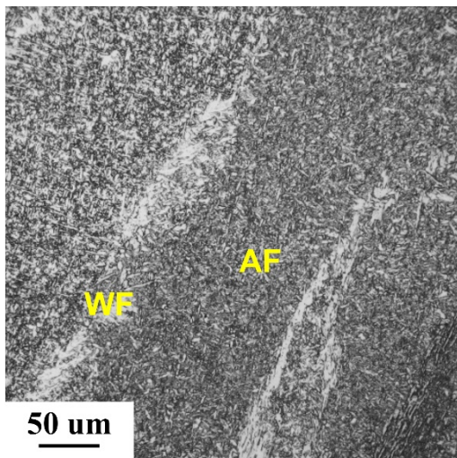
Fig.9. Microstructure of weld metal by FCAW.
