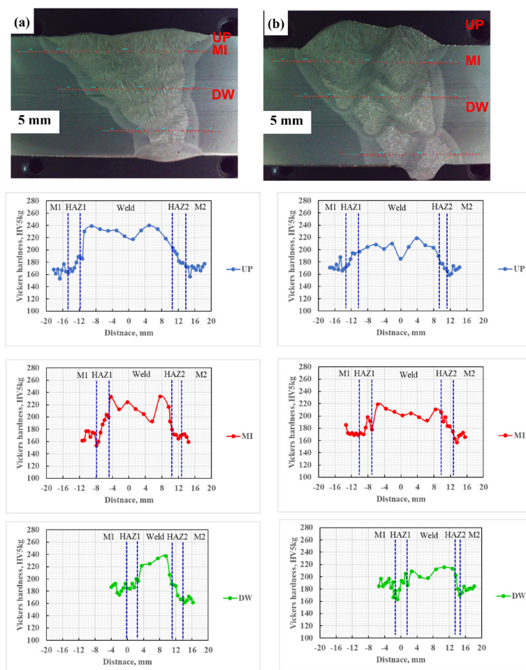
Fig.13. The macro-metallography of weldment and hardness distribution of (a) FCAW and (b) MCAW weldment
