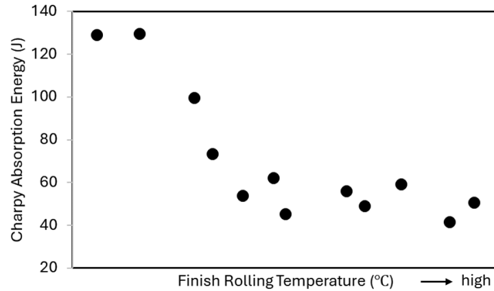
Fig.4. Influences of finish rolling temperature on the (L-T) Charpy absorption energy of AR400F at -40^\circ\text{C} .
