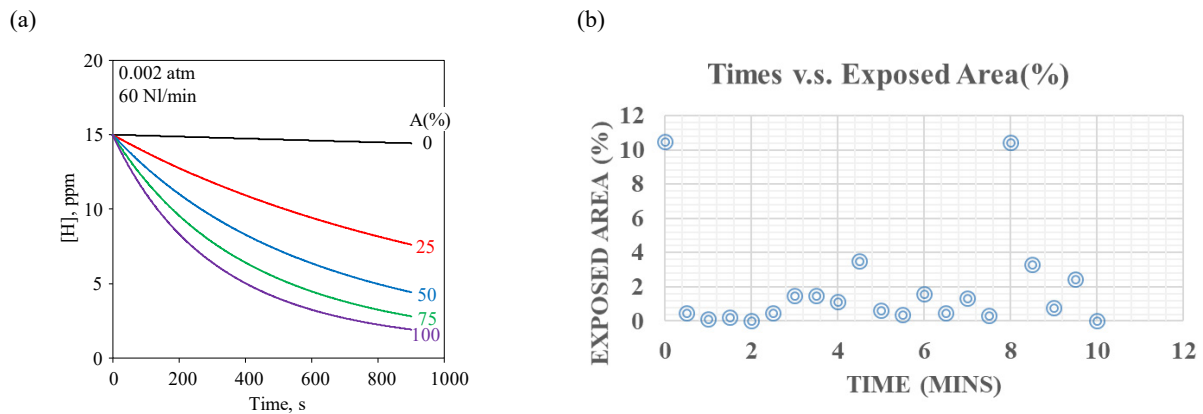
Fig.4. (a) Effect of a fraction of exposed area at the top surface ( A(\%) ) on change of [H] with time in VD process, (b) the proportion of molten steel exposed area on the pinhole detection surface changes with time.
