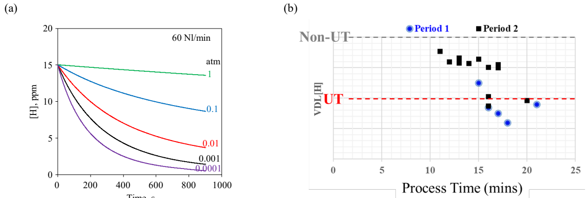
Fig.2. (a) The effect of vacuum chamber pressure on [H] with time; (b) the effect of dehydrogenation process time on VDL[H] .
